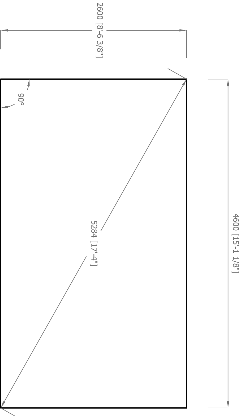
Base Plan
